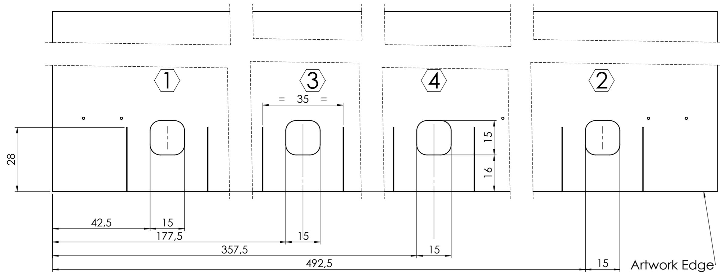
- Detail 1 Holes made by punching pliers
