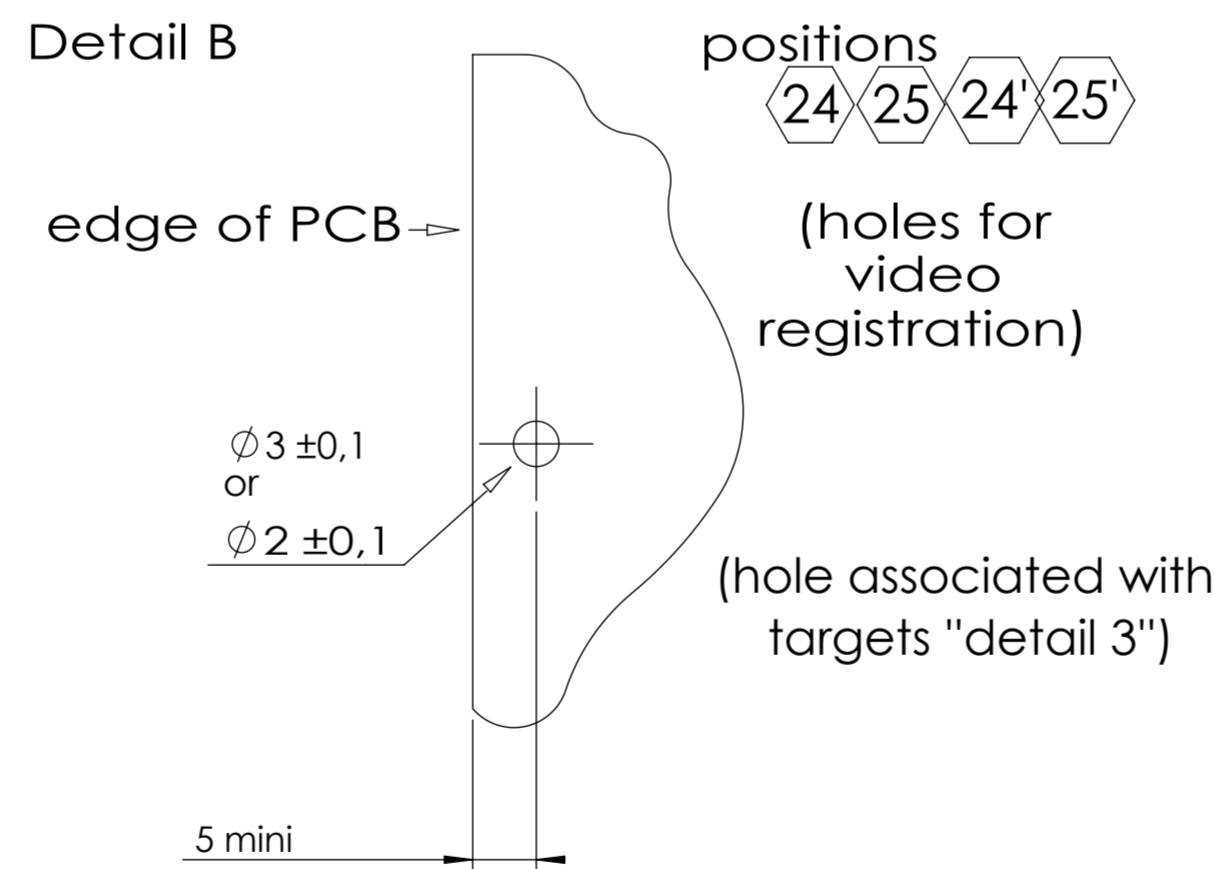
Details of the the PCB
